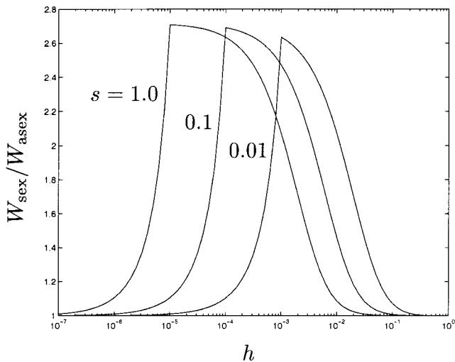
FIGURE 5.—Ratio of the mean fitness of the sexual population to that of the asexual population vs. the dominance h for three representative values of s . We have assumed u = 10^{-5} and n = 10^5 so that U = 1.0 .
