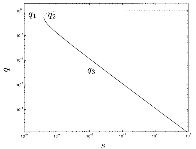
FIGURE 3.—Bifurcation diagram varying s for fixed h = 0.9 , u = 10^{-5} .
