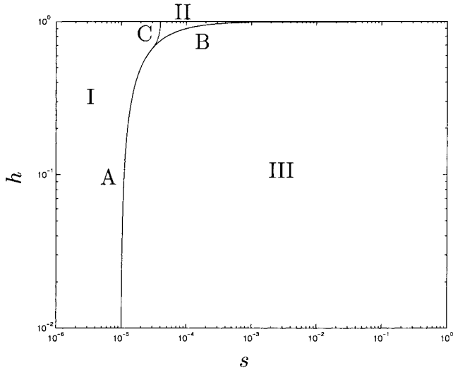
FIGURE 1.—Regions in the s - h parameter space with different sexual solutions of the mutation-selection balance equations. The mutation rate is taken as u = 10^{-5} .
