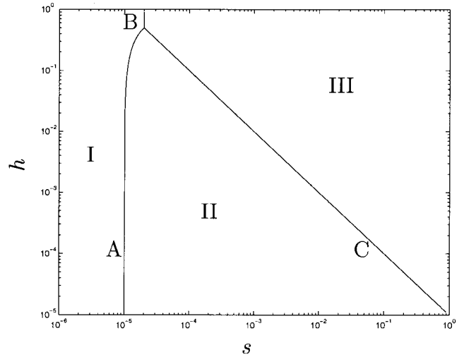
FIGURE 4.—Regions in the s - h parameter space for which three different asexual solutions of the mutation-selection balance equations are stable. The mutation rate is taken as u = 10^{-5} .
