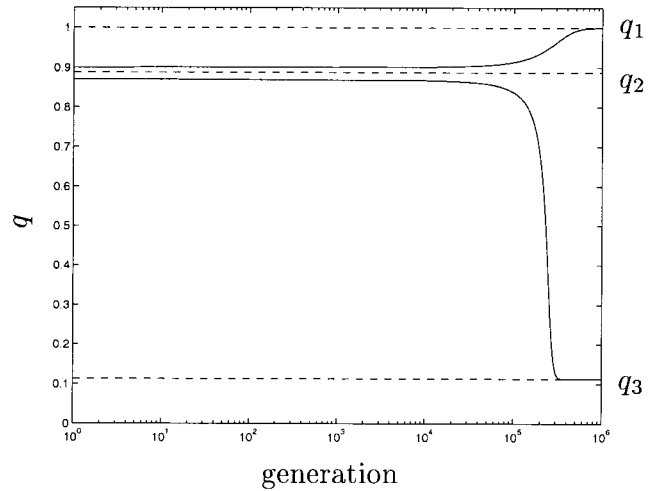
FIGURE 2.—Evolution of q in region II of Figure 1 with initial conditions above and below q_2 . Dashed lines are the analytical equilibrium solutions and solid lines are the numerical results. Here, u = 10^{-5} , h = 1.0 , and s = 10^{-4} .
