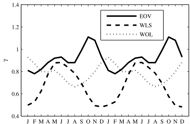
Figure 14. Seasonal cycle of the stratification ratio for EOV, WLS, and WOL.
