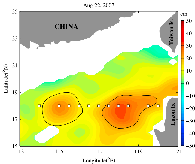
Figure 1. SLA distribution (color) on 22 August 2007. White squares denote the CTD locations. Black contour marks the edge of an eddy. The altimetry data over the shelf shallower than 500 m is discarded.
