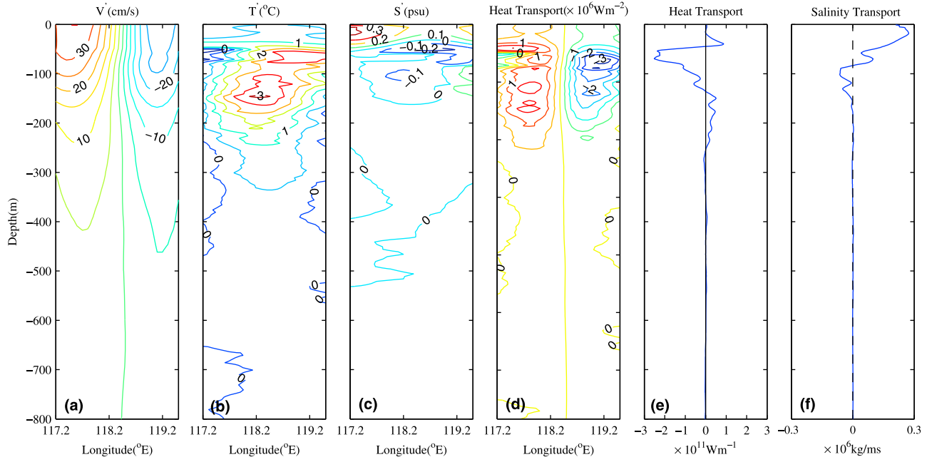
Figure 3. (a) Meridional geostrophic flow (cm/s); (b) temperature anomaly ( ^{\circ}\text{C} ); (c) salinity anomaly (psu); (d) heat transport ( \rho C_p \nu' T' ) distribution associated with the anticyclonic eddy next the Luzon Island detected on 22 August 2007; (e) heat transport integrated across the eddy; and (f) salt transport integrated across the eddy.
