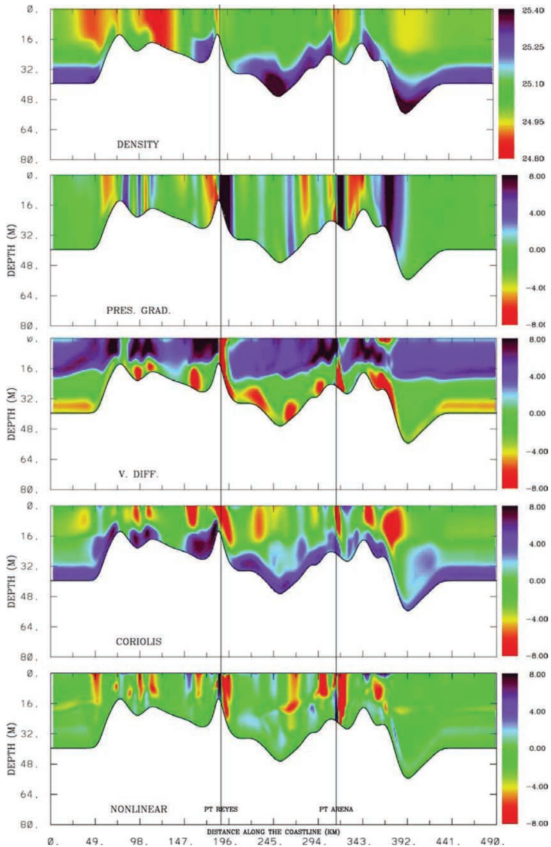
Figure 13. Potential density \sigma_\theta (kg m -3 ) and terms from the alongshore momentum equation (1): pressure gradient, vertical diffusion, Coriolis force, and nonlinear advection (m s -2 , averaged over 24 hrs, multiplied by 10 6 ) as a function of depth and distance along the coast at locations approximately 2.5 km offshore on day 3.
