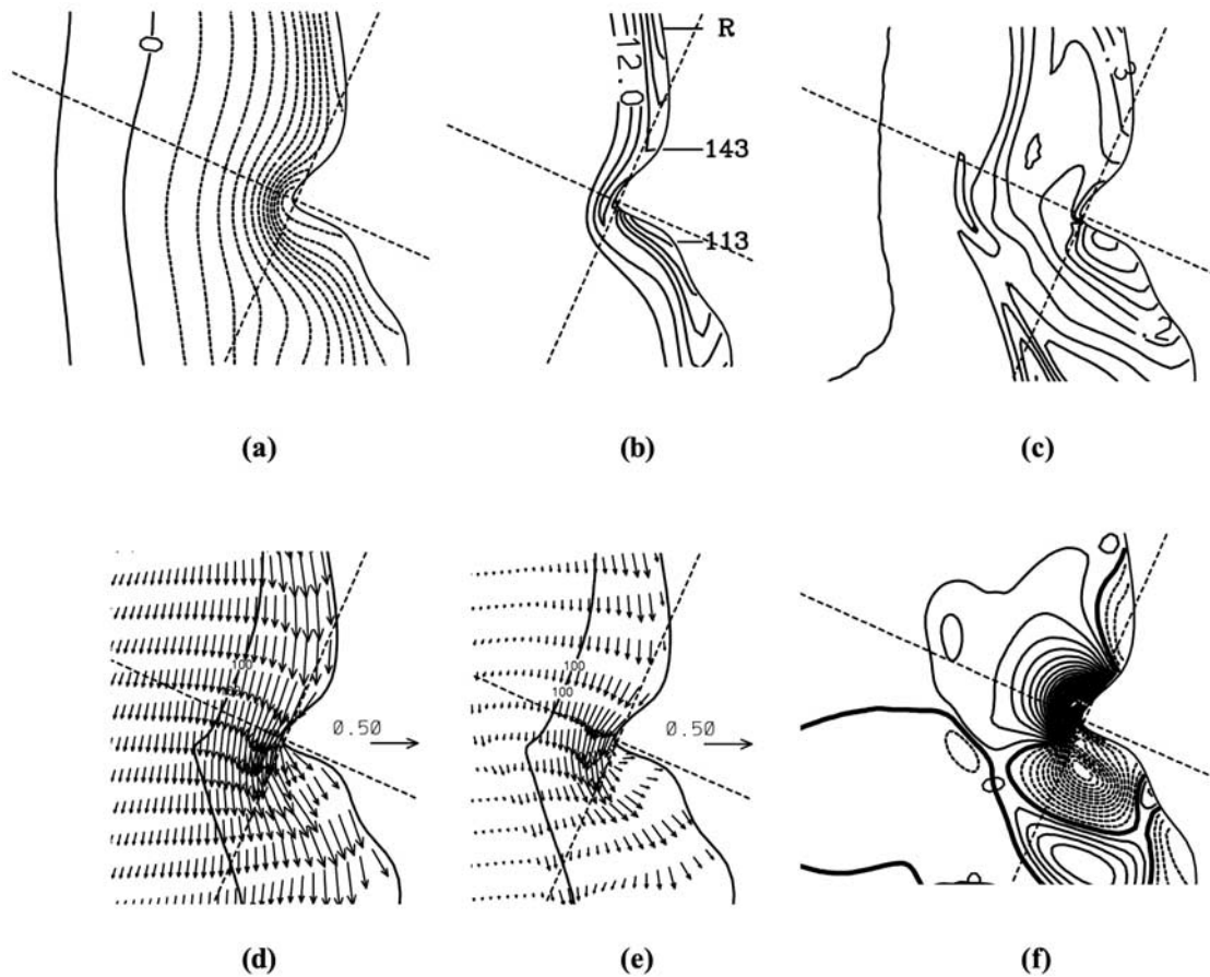
Figure 11. Daily averaged fields on day 3 of (a) surface elevation (interval 0.5 cm), (b) surface temperature (interval 0.2 C), (c) \sigma_\theta - \sigma_\theta(t=0) at the bottom (interval 0.05 kg m -3 ), (d) surface velocity vectors (m s -1 ), (e) velocity vectors (m s -1 ) at \sigma = -0.658 , and (f) depth-averaged y pressure gradient (multiplied by 10 6 ; interval 1 m s -2 with a heavy contour line for 0).
