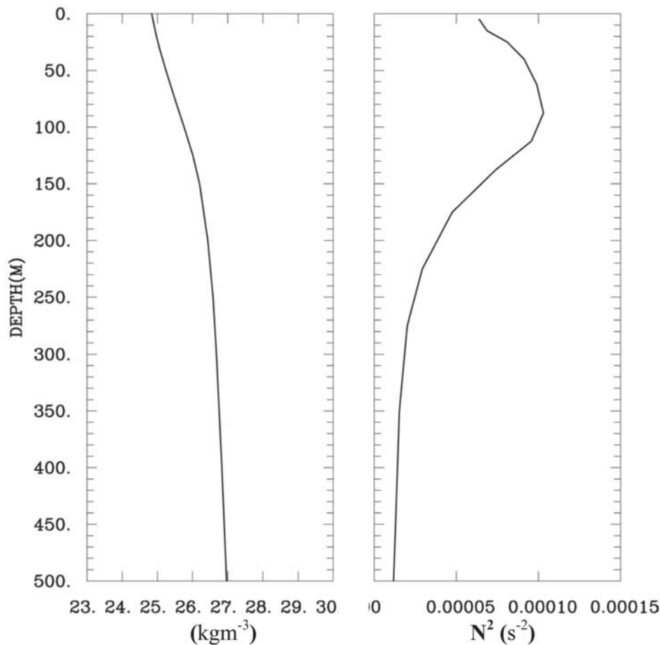
Figure 4. Initial values of \sigma_\theta and N^2 as a function of depth.
