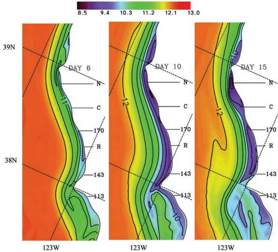
Figure 5b. Surface temperature (°C) on days 6, 10, and 15. The contour interval is 0.5°C.
