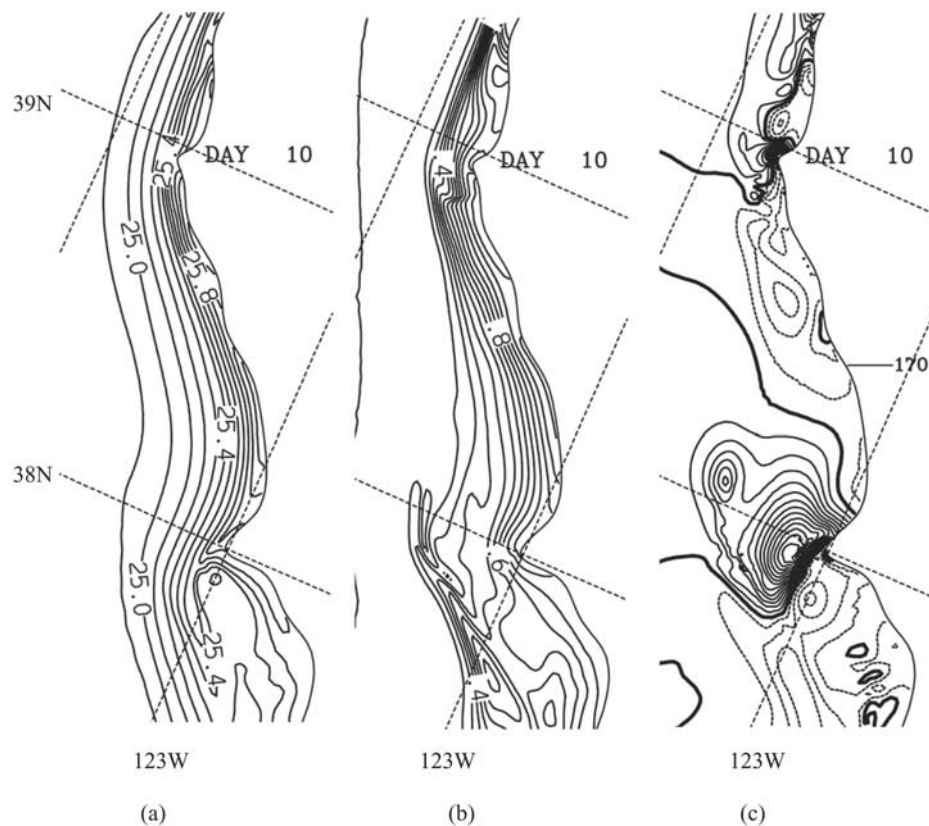
Figure 18. Daily averaged fields on day 10 of (a) \sigma_\theta at the surface (interval 0.1 \text{ kg m}^{-3} ), (b) \sigma_\theta - \sigma_\theta(t = 0) at the bottom (interval: 0.05 \text{ kg m}^{-3} ), and (c) depth-averaged y pressure gradient (multiplied by 10^6 , interval 1 \text{ m s}^{-2} with a heavy contour line for 0).
