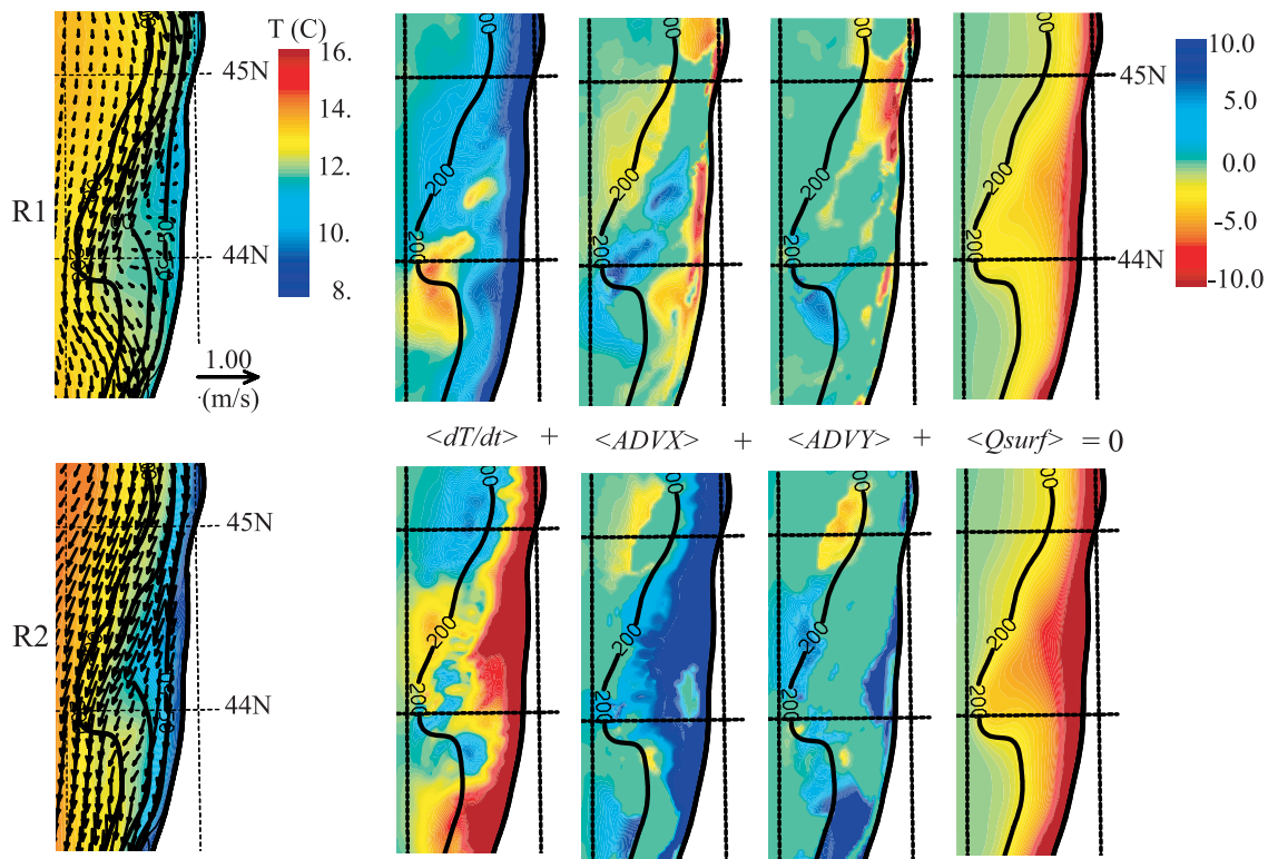
Figure 19. Fields of time mean surface velocity vectors ( \text{m s}^{-1} ), surface temperature ( ^{\circ}\text{C} ), and time-averaged values of terms ( \text{C s}^{-1} , multiplied by 10^{-7} ) in the depth-averaged temperature equation calculated as described in Appendix A: \langle ADVY \rangle alongshore advection, \langle ADVX \rangle across-shore advection, \langle dT/dt \rangle time rate of temperature change and \langle Q_{surf} \rangle surface heat flux. The time-averaged periods are 3–12 June for regime 1 (R1), dominated by northward wind forcing, and 1–10 July for regime 2 (R2), dominated by southward wind forcing.
