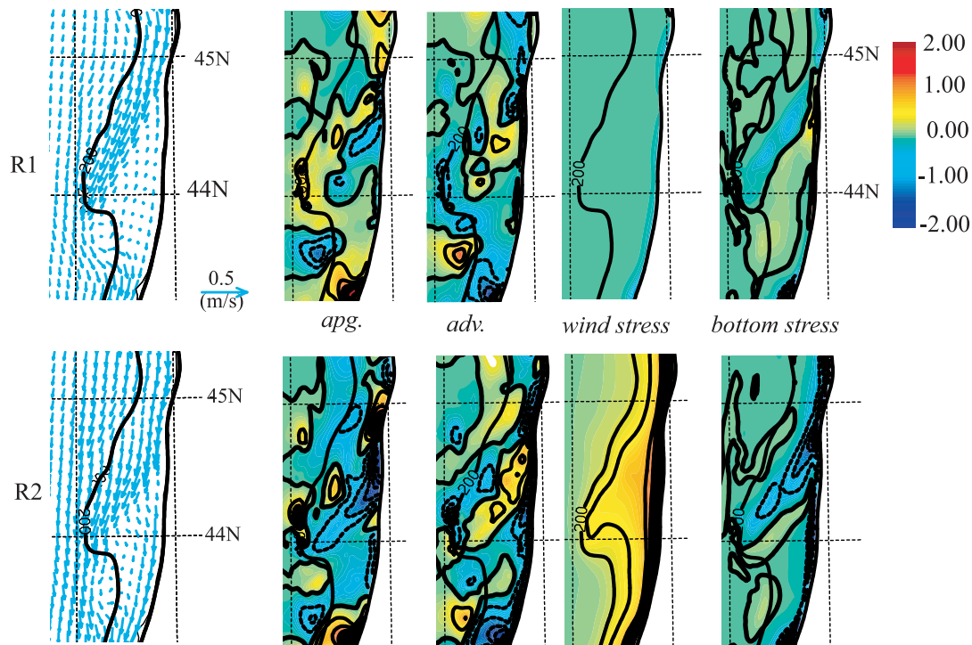
Figure 16. Fields of time mean depth-averaged velocity vectors ( \text{m s}^{-1} ) and time mean fields of term from the depth-averaged alongshore momentum equation: apg, ageostrophic pressure gradient; adv, nonlinear advection; wind stress; and bottom stress (divided by water depth and multiplied by 10^6 \text{ m s}^{-2} ). The time averaged periods are 3–12 June for regime 1 (R1), dominated by northward wind forcing, and 1–10 July for regime 2 (R2), dominated by southward wind forcing.
