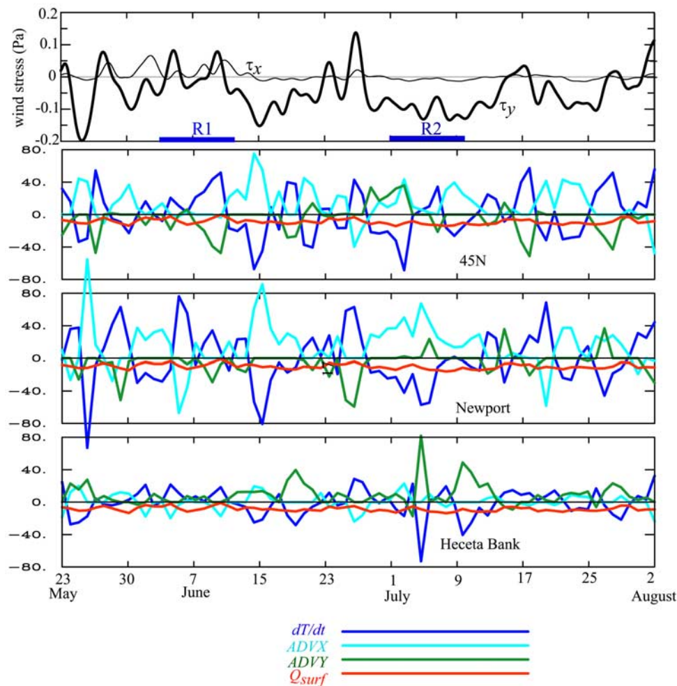
Figure 20. Time series of terms in the depth-averaged temperature equation ( Cs^{-1} , multiplied by 10^{-7} ) calculated as described in Appendix A at about 8 km offshore at 45^{\circ}\text{N} (line 200, water depth 64 m), Newport (line 175, water depth 58 m), and Heceta Bank (line 148, water depth 63 m). The corresponding time series of wind stress near Newport is also shown.
