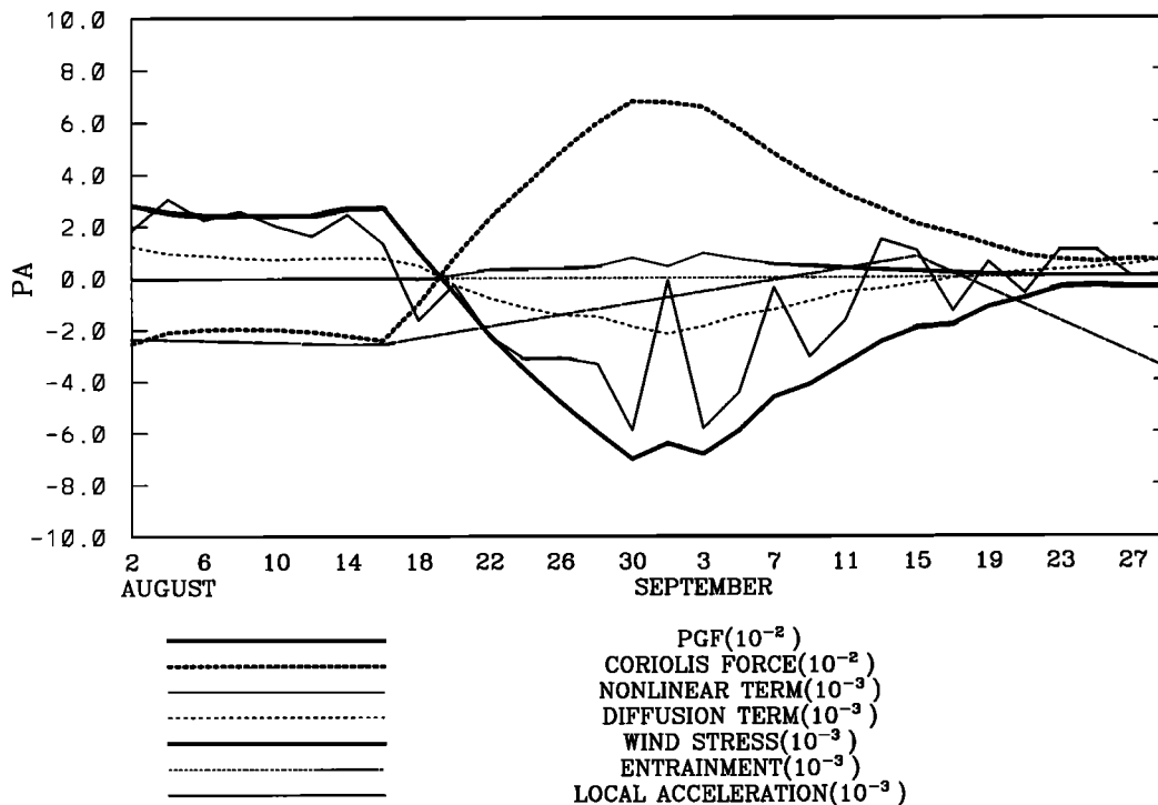
Figure 7. Time series of the N-S momentum balance in G_1 in the north end of profile A. PGF, -h_1 \rho_0 \partial P_1 / \partial y ; Coriolis force, -f h_1 u_1 \rho_0 ; nonlinear term, \rho_0 \nabla \cdot (h_1 v_1 \mathbf{v}_1) ; diffusion term, -\rho_0 K_u \nabla \cdot (h_1 \nabla v_1) ; wind stress, -\tau_y ; entrainment term, -W_e [H(W_e) v_2 + H(-W_e) v_1] \rho_0 . Positive value refers to the northward direction.
