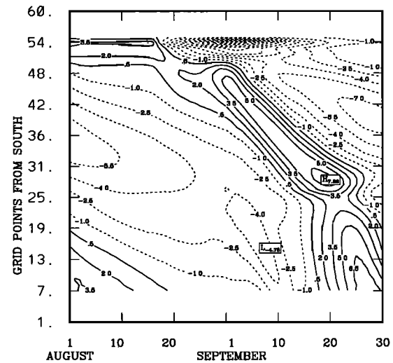
Figure 9. Time series of vorticity ( 10^{-6} \text{ s}^{-1} ) along profile A in G_1 .
