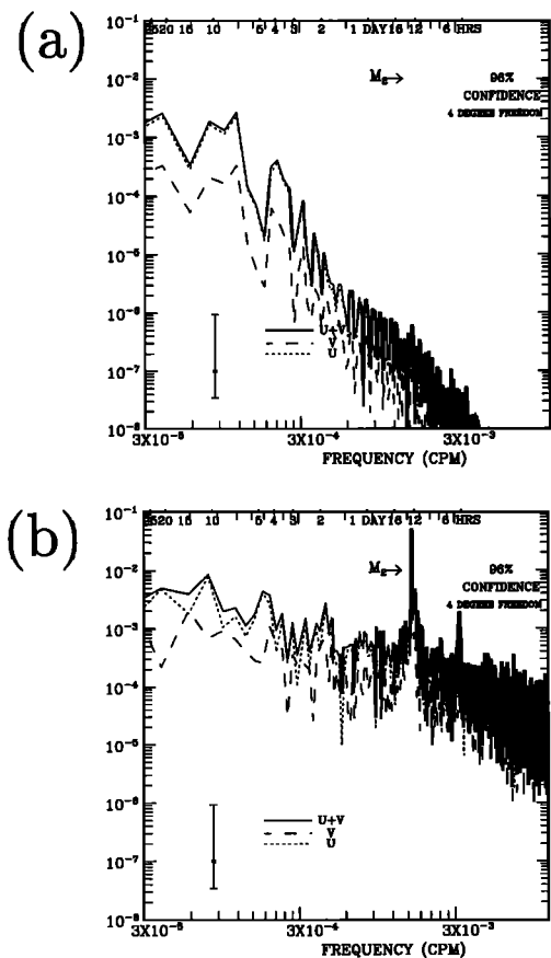
Figure 4. Energy spectra of (a) simulated and (b) observed velocity at station Bonaventure. Ordinate units are u^2/s^2 .
