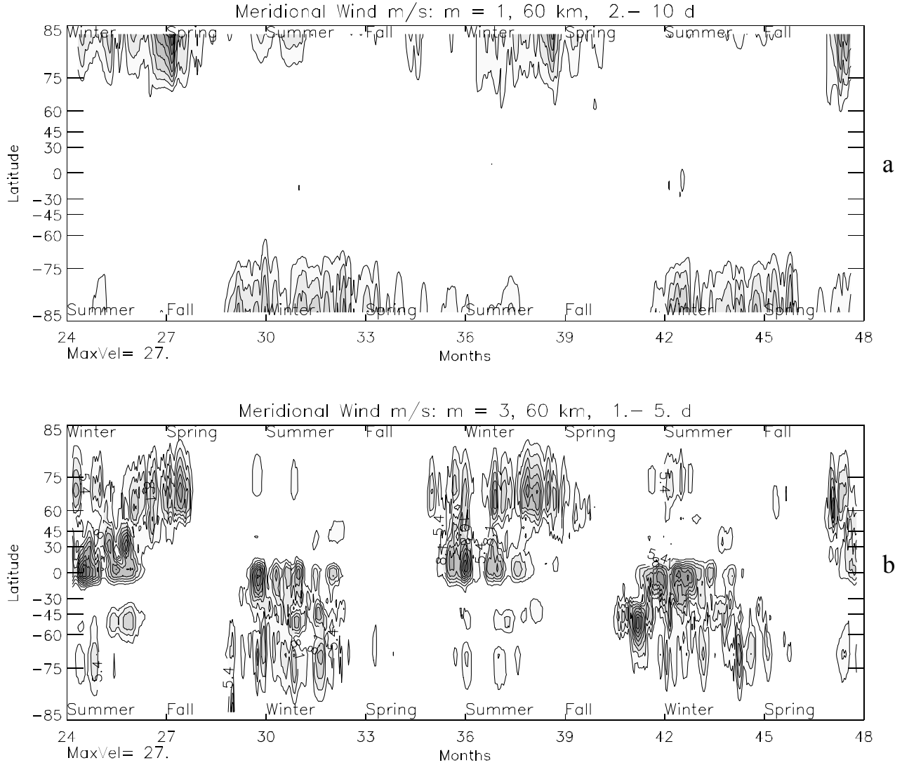
Fig. 11. Computed seasonal variations of meridional winds at 60 km for planetary waves with zonal wave numbers m=1 and 3. The resemblance with the seasonal variations of the IGWs in Fig. 8 indicates that both classes of waves have similar roots as discussed in the main text.
